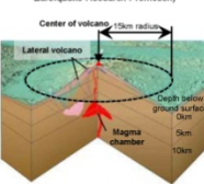
Example of the relationship between the center of a volcano and lateral volcanoes, etc. (in the case of polygenetic volcano) (modified from the "Siting Factors for the Selection of Preliminary Investigation Areas," NUMO, 2009)
