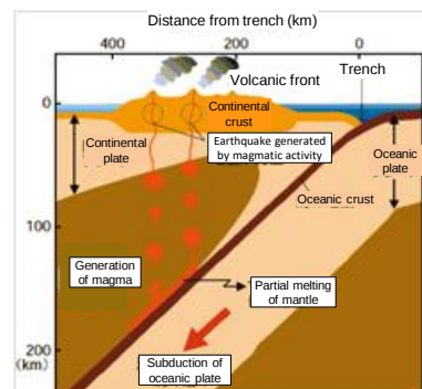
Plate subduction and volcanic activity (modified from the Headquarters for Earthquake Research Promotion)
