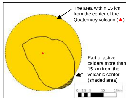
Example of mapping calderas where the area of Quaternary volcanic activity exceeds 15 km (for the case of Kikai)
