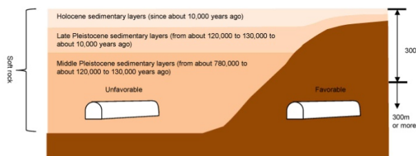
Schematic illustration of unconsolidated sediments
