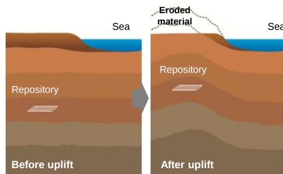
Schematic illustration of uplift/erosion
