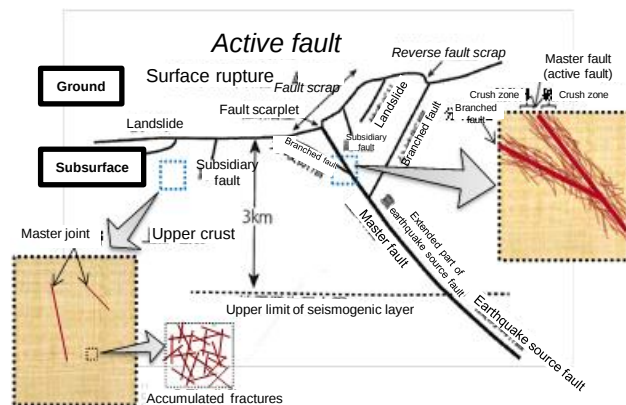
Various appearance forms of an active fault, etc. (modified from Yamazaki, 2013)
