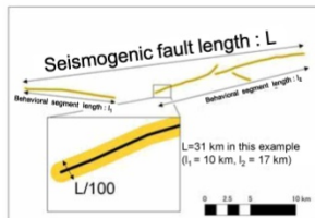
Example of mapping width of 1/100 of a seismogenic fault length (in the case of the seismogenic fault of Mount Naqi)
