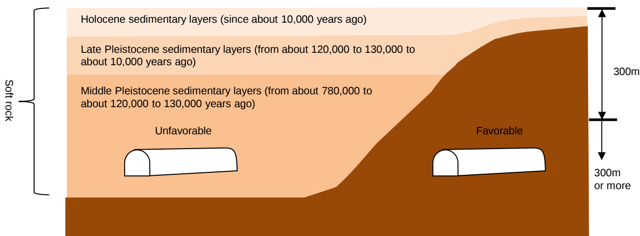
Schematic illustration of unconsolidated sediments
