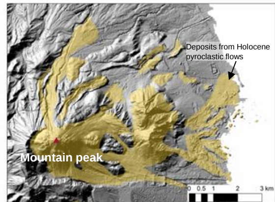
Example of mapping the distribution of deposits from Holocene pyroclastic flows at Mount Unzen
