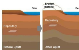
Schematic illustration of uplift/erosion
