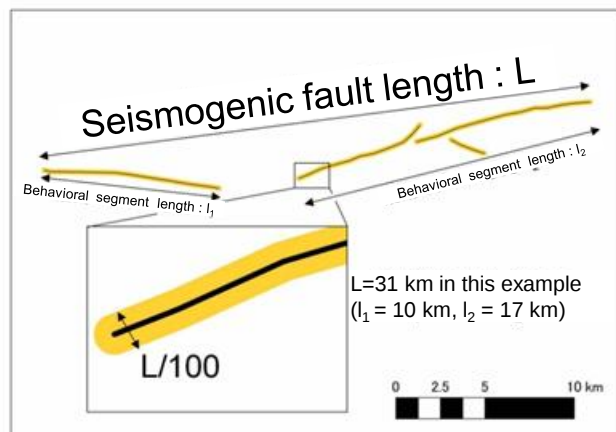
Example of mapping width of 1/100 of a seismogenic fault length (in the case of the seismogenic fault of Mount Nagi)
