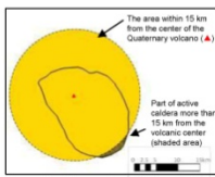
Example of mapping calderas where the area of Quaternary volcanic activity exceeds 15 km (for the case of Kikai)
