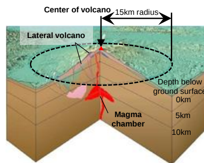
Example of the relationship between the center of a volcano and lateral volcanoes, etc. (in the case of polygenetic volcano)
