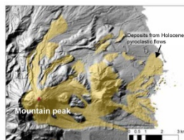
Example of mapping the distribution of deposits from Holocene pyroclastic flows at Mount Unzen (from the website of the AIST: The Seamless Digital Geological Map of Japan (1:200,000) and Geospatial Information Authority of Japan: shaded relief image)
