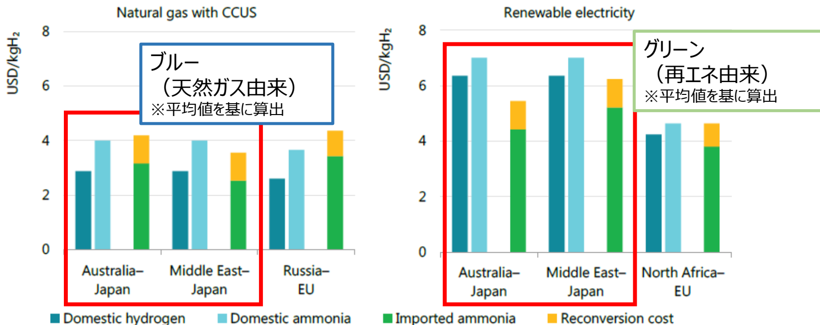
Figure 31. Comparison of delivered hydrogen costs for domestically produced and imported hydrogen for selected trade routes in 2030
